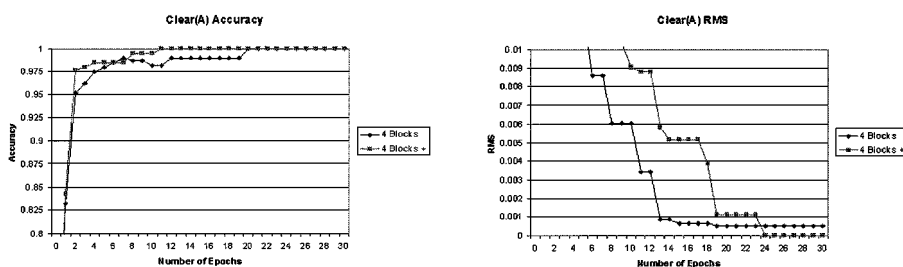
Figure 14. Learning curves for the goal clear(a) in the 4 blocks world. The curves denoted with + are obtained using an additional background knowledge predicate.
